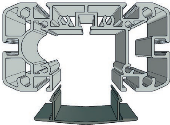
Close-up: support extrusions center column cable channel
